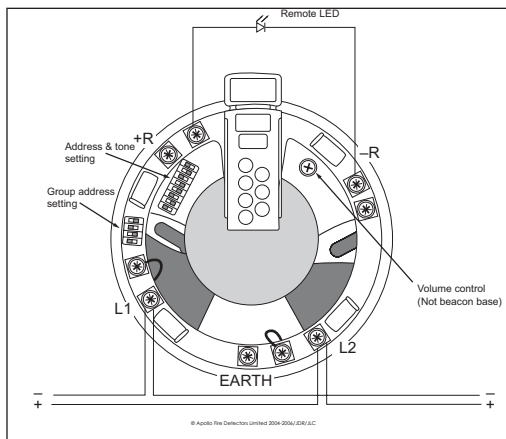
Fig. 2 Sounder Beacon Base wiring
