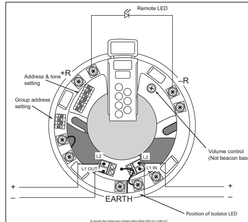
Fig. 3 Sounder Beacon Base with isolator wiring
